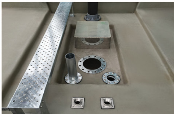
Cold Water Basin Connection
