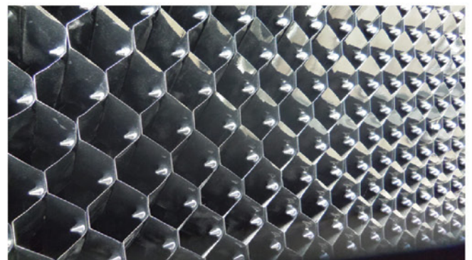
Adhesire Free UPVC Fill Sheet With Interlocking Studs
